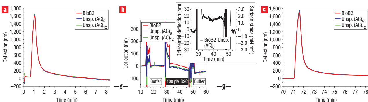
Figure 2 Calibration of the mechanical response and the biosensitivity of the cantilever array sensors. a,b , Calibration by application of a heat pulse of 0.7 °C for 30 s ( a ), followed by 100 pM complementary BioB2 cDNA injection ( b ), which results in compressive stress due to hybridization of the specific complementary cDNA with an absolute signal of ~17 nm. Inset: The differential signal is evaluated by subtracting the response of the Unsp. (AC) 6 -sensitized cantilever from the signal of the BioB2-sensitized cantilever. c , Cantilever sensor calibration by applying a heat pulse after the sensitivity-validation experiment. This demonstrates the mechanical stability and integrity of the sensors.
