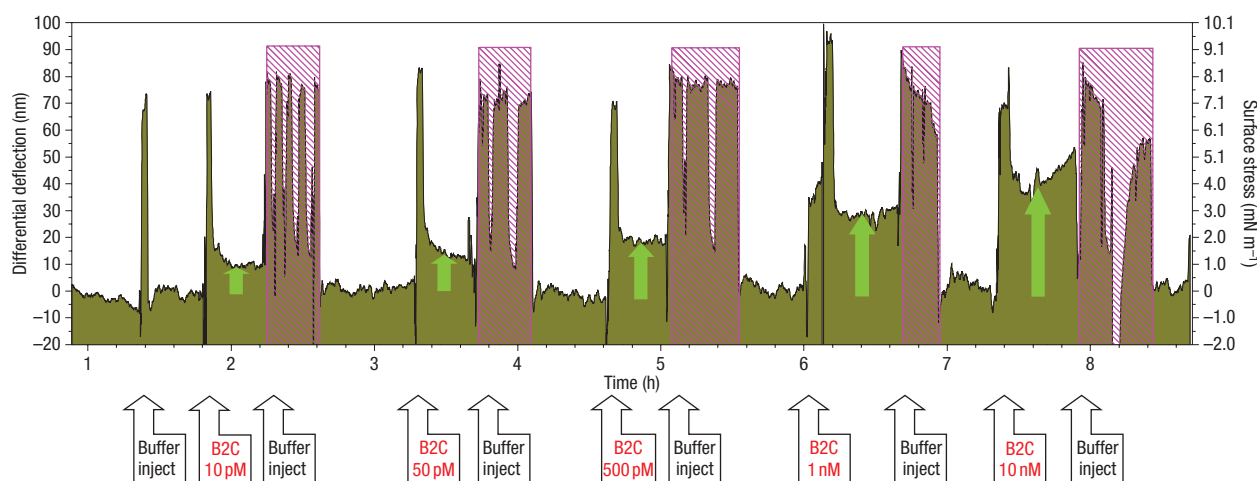
Figure 3 Cantilever response as function of BioB2C concentration. A series of continuous injections of increasing concentrations (10 pM to 10 nM) of complementary ssDNA B2C is shown. During buffer injection the sensors are flexed owing to flow. Dehybridization of the hybridized target (red hatched areas) occurs owing to the short length of the BioB2 oligonucleotides (12mer, see Table 1).
