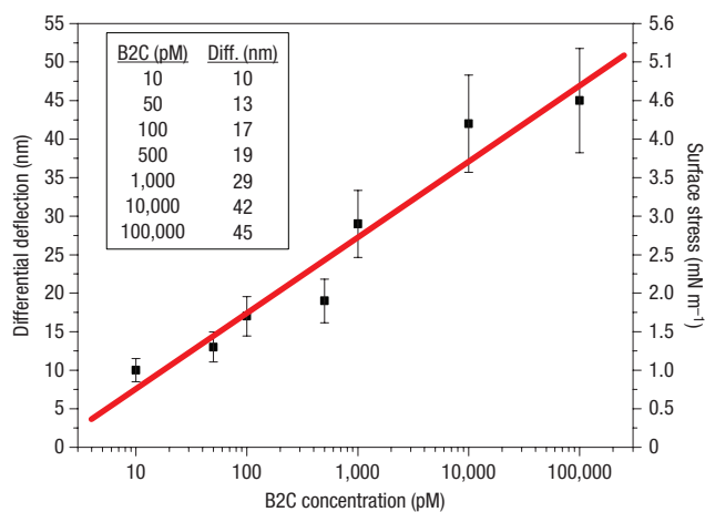
Figure 4 Differential nanomechanical response of cantilevers during specific hybridization. Compressive stress response versus concentration dependence. The error bars represent standard deviation obtained from four measurements.
